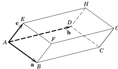
Section 9.1. Parallelepiped in Team Project 38(f)
