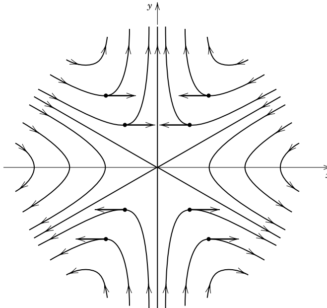
Section 18.4. Problem 8
