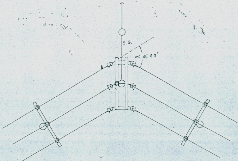
PRIMARY STUB GUY, FOR MEDIUM ANGLES
