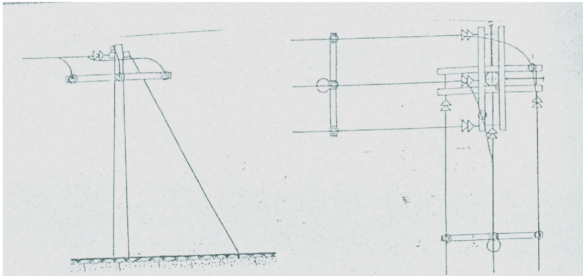
PRIMARY, TWO DOWN GUYS FOR LARGE ANGLES & HIGHER TENSIONS
