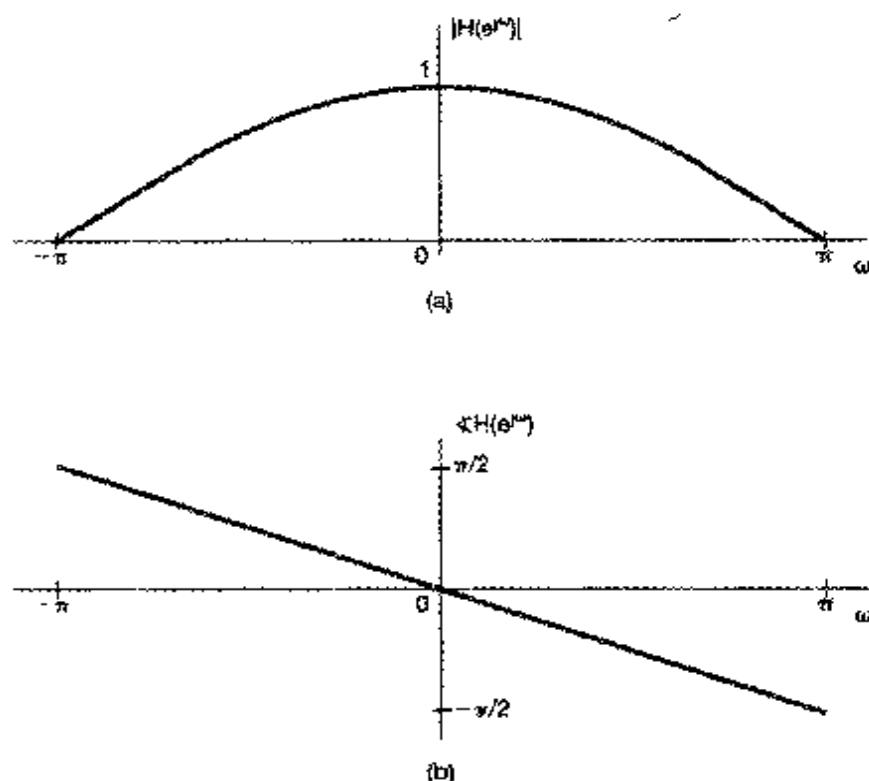
Figure 3.2S (a) Magnitude and (b) phase for the frequency response of the discrete-time LTI system y[n] = 1/2(x[n] + x[n-1]) .
