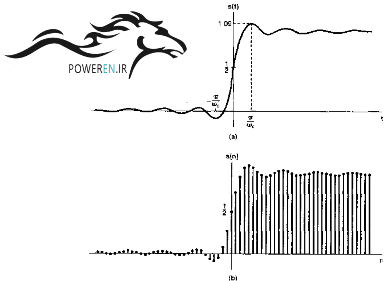
Figure 6.14 (a) Step response of a continuous-time ideal lowpass filter, (b) step response of a discrete-time ideal lowpass filter.
