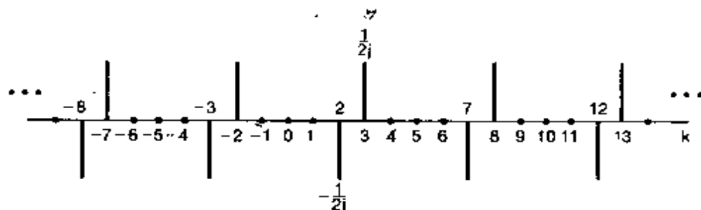
Figure 3.14 Fourier coefficients for x[n] = \sin 3(2\pi/5)n .
