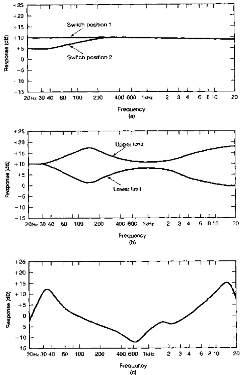
Figure 3.22 Magnitudes of the frequency responses of the equalizer circuits for one particular series of audio speakers, shown on a scale of 20 \log_{10} |H(j\omega)| , which is referred to as a decibel (or dB) scale. (a) Low-frequency filter controlled by a two-position switch; (b) upper and lower frequency limits on a continuously adjustable shaping filter; (c) fixed frequency response of the equalizer stage.
