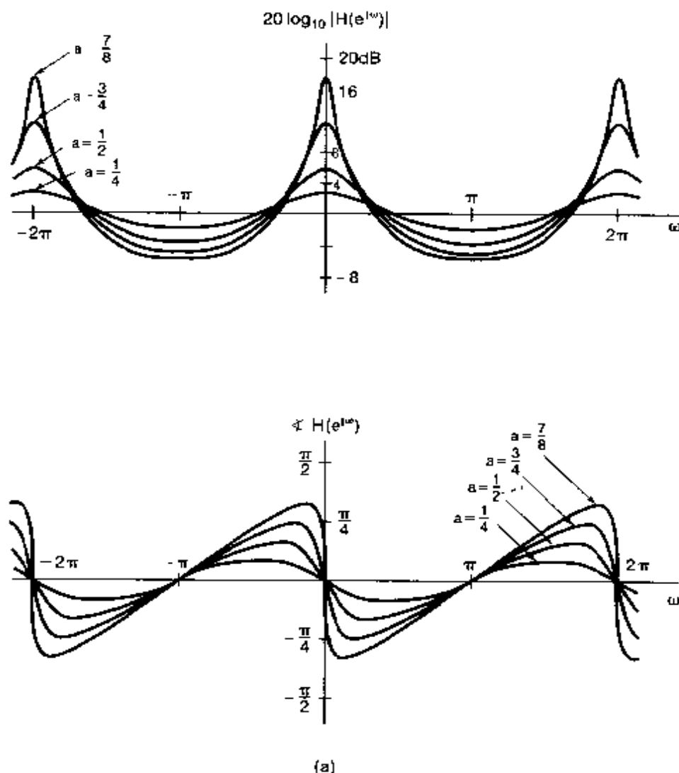
Figure 6.28 Magnitude and phase of the frequency response of eq. (6.52) for a first-order system: (a) plots for several values of a > 0 ; (b) plots for several values of a < 0
