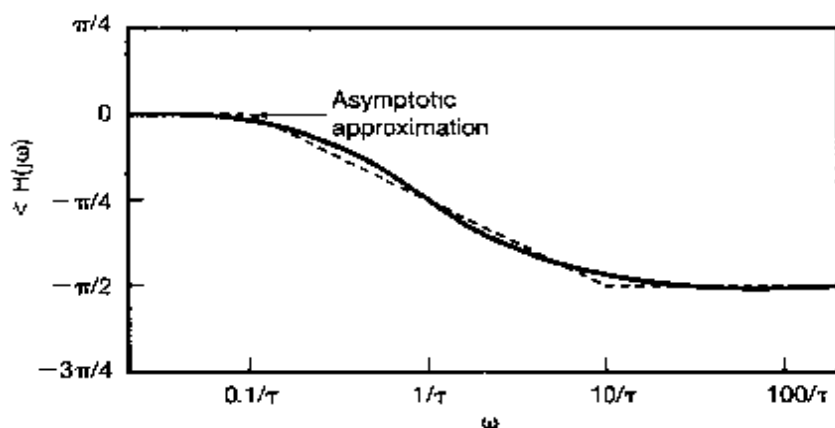
Figure 6.20 Bode plot for a continuous-time first-order system.
