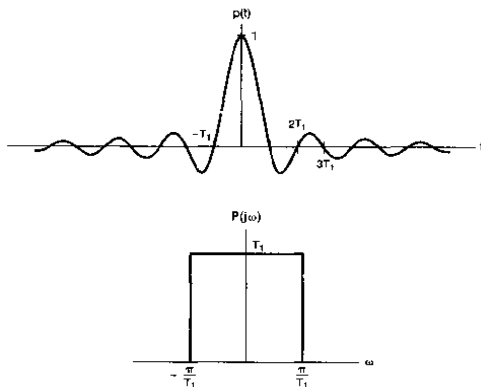
Figure 8.29 A sinc pulse and its corresponding spectrum.
