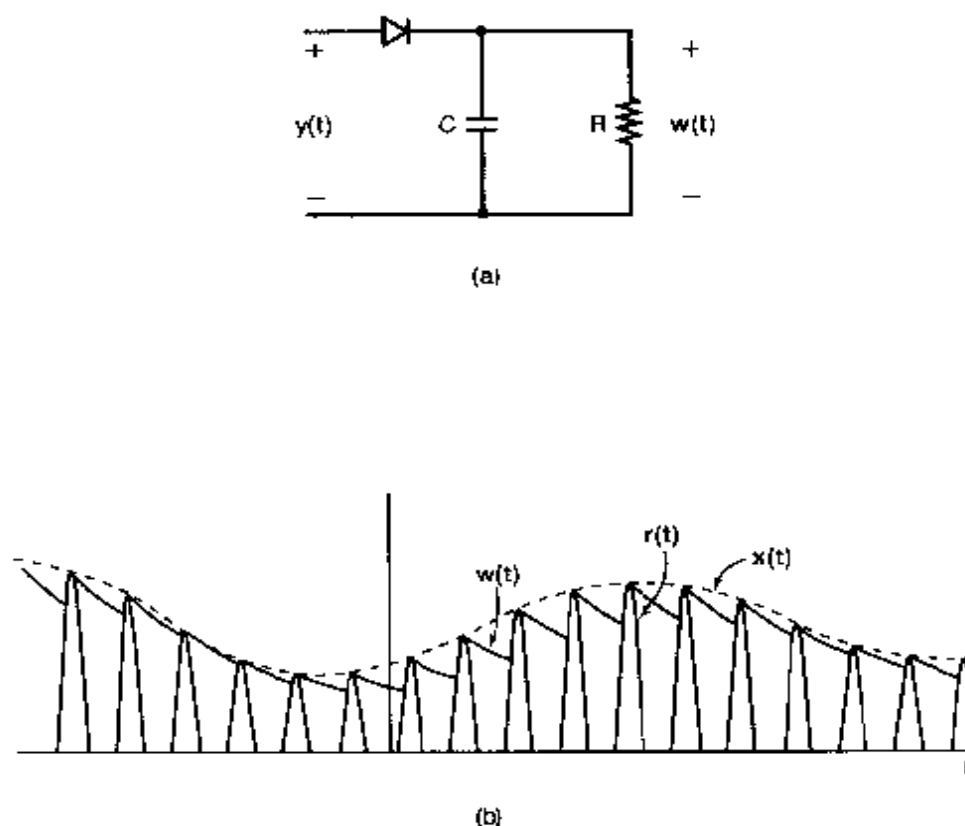
Figure 8.11 Demodulation by envelope detection (a) circuit for envelope detection using half-wave rectification; (b) waveforms associated with the envelope detector in (a): r(t) is the half-wave rectified signal, x(t) is the true envelope, and w(t) is the envelope obtained from the circuit in (a). The relationship between x(t) and w(t) has been exaggerated in (b) for purposes of illustration. In a practical asynchronous demodulation system, w(t) would typically be a much closer approximation to x(t) than depicted here.
