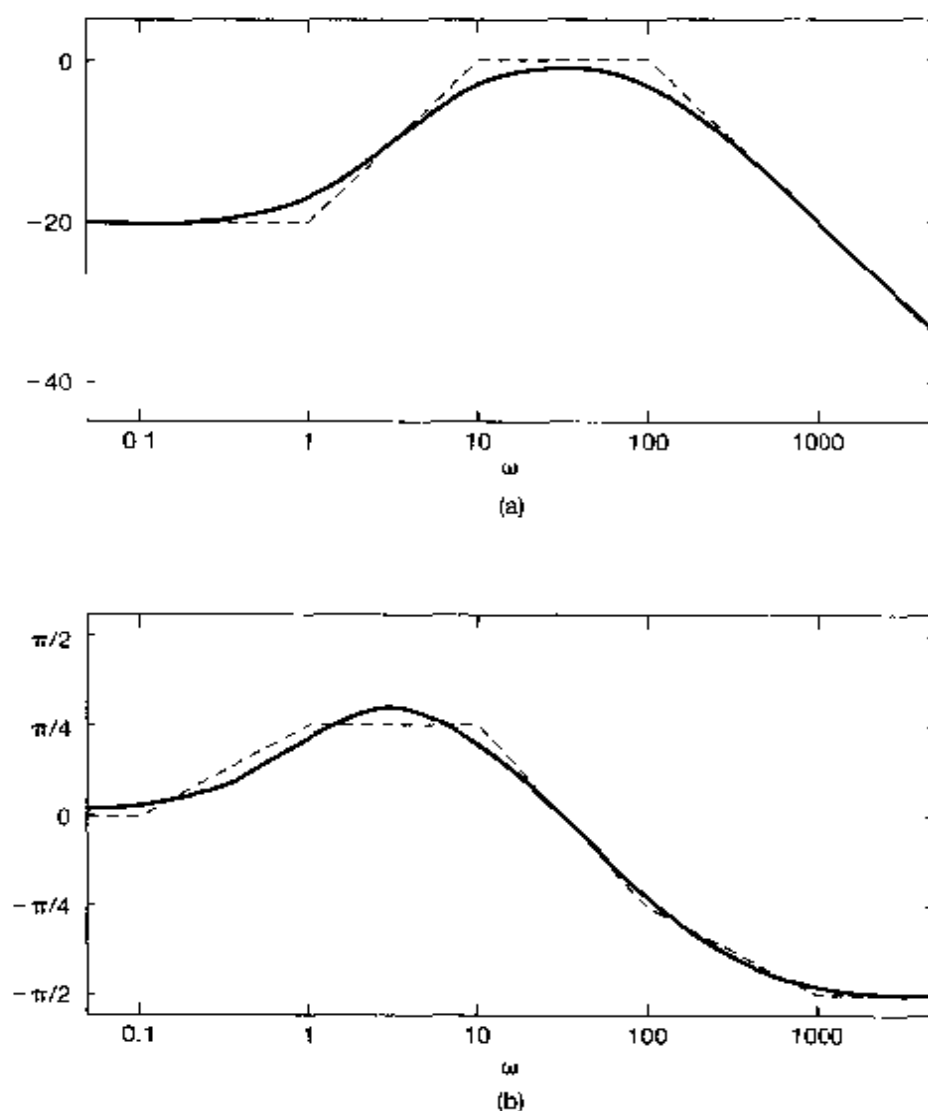
Figure 6.25 Bode plot for system function in Example 6.5: (a) magnitude; (b) phase.
