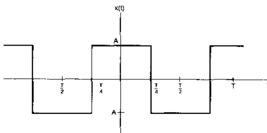
Figure 8.36 Symmetric periodic square wave.
