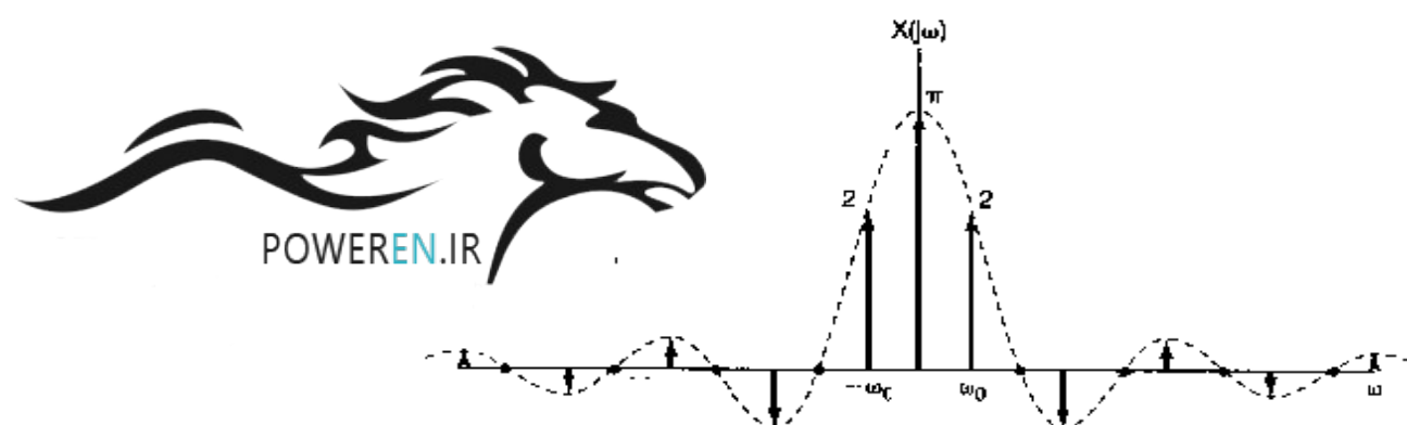
Figure 4.12 Fourier transform of a symmetric periodic square wave
