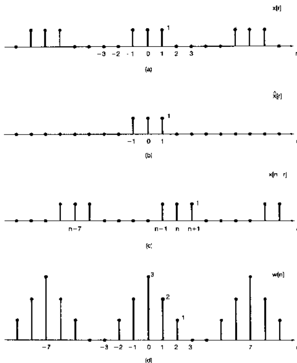
Figure 3.21 (a) The square-wave sequence x[r] in Example 3.15; (b) the sequence \hat{x}[r] equal to x[r] for -3 \leq r \leq 3 and zero otherwise; (c) the sequence x[n-r] ; (d) the sequence w[n] equal to the periodic convolution of x[n] with itself and to the aperiodic convolution of \hat{x}[n] with x[n] .
