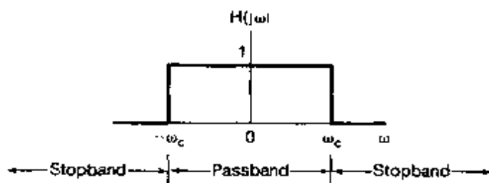
Figure 3.26 Frequency response of an ideal lowpass filter.
