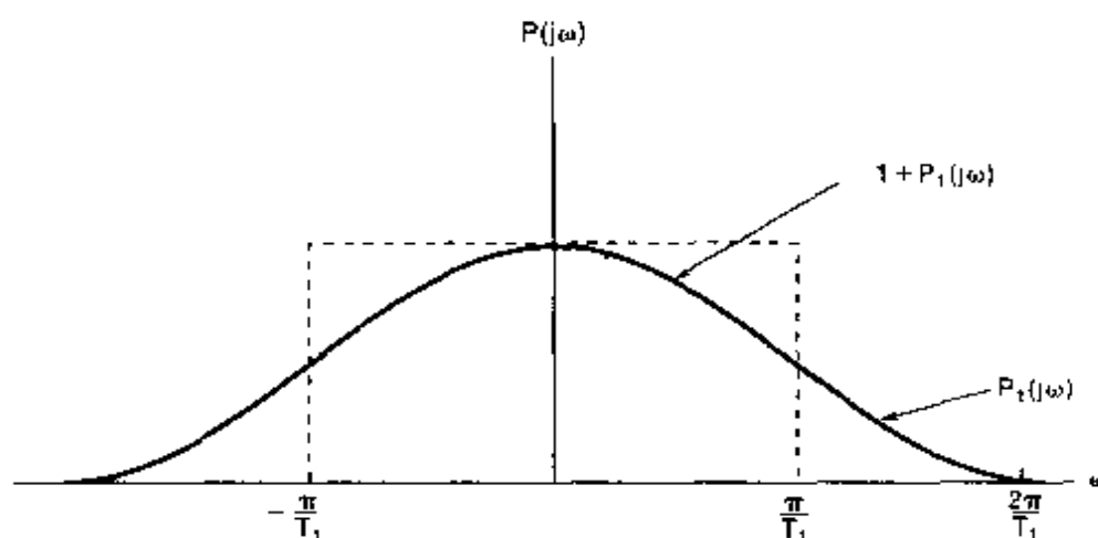
Figure 8.31 Odd symmetry around \pi/T as defined in eq. (8.29).
