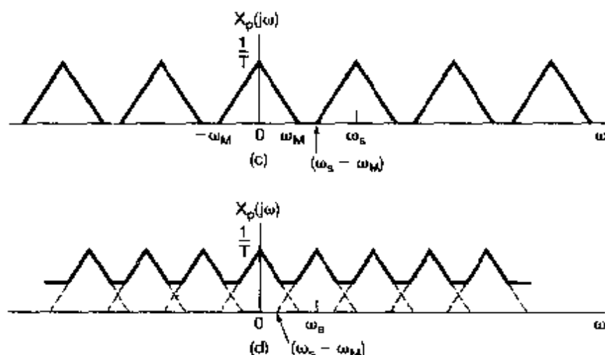
Figure 7.3 Continued (c) spectrum of sampled signal with \omega_s > 2\omega_M ; (d) spectrum of sampled signal with \omega_s < 2\omega_M .
