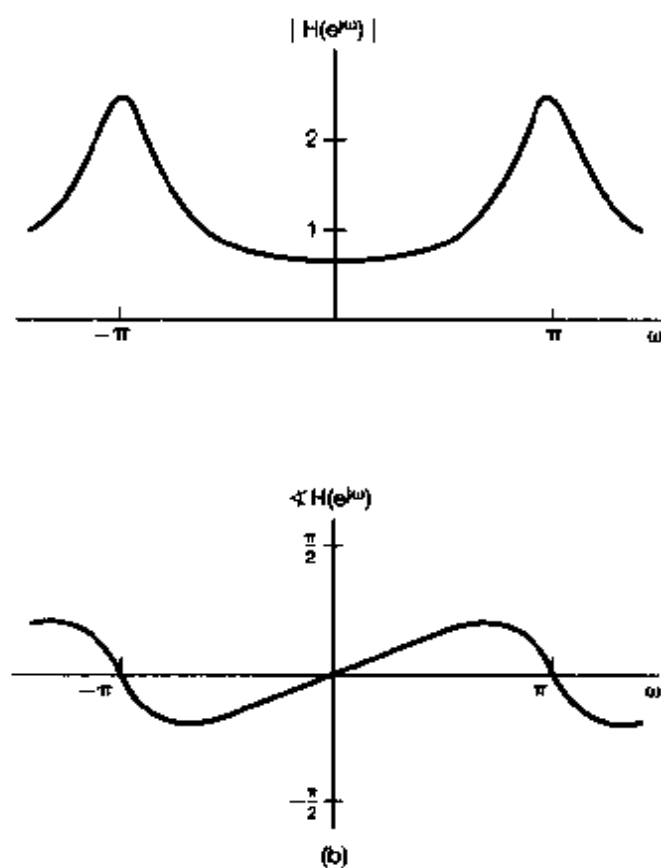
Figure 3.34 Frequency response of the first-order recursive discrete-time filter of eq. (3.151): (a) a = 0.6 ; (b) a = -0.6 .
