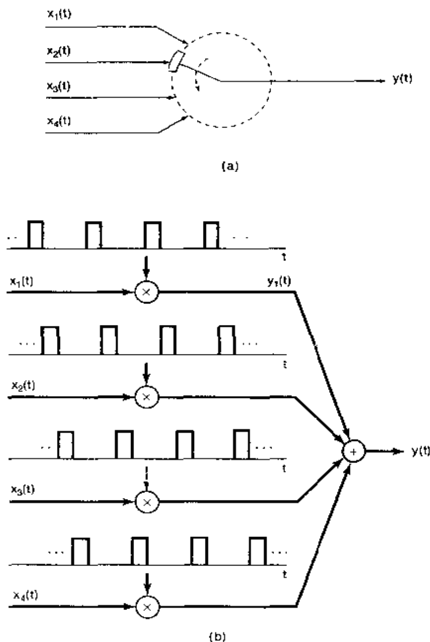
Figure 8.25 Time-division multiplexing.
