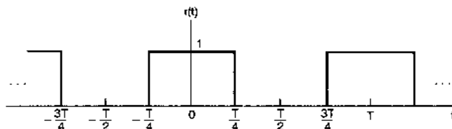
Figure 8.38 Symmetric square wave r(t) in eq. (8.50).
