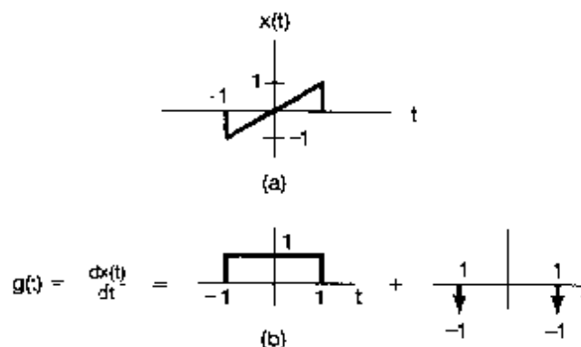
Figure 4.16 (a) A signal x(t) for which the Fourier transform is to be evaluated; (b) representation of the derivative of x(t) as the sum of two components.
