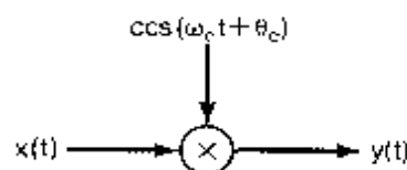
Figure 8.3 Amplitude modulation with a sinusoidal carrier.
