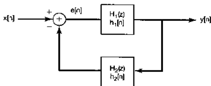
Figure 10.17 Feedback interconnection of two systems.
