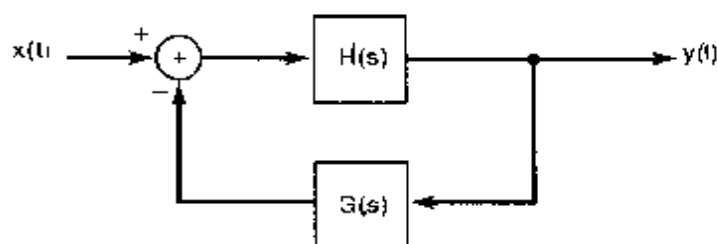
Figure 11.25 Typical feedback system designed to be stable, assuming nominal descriptions for H(s) and G(s) .
