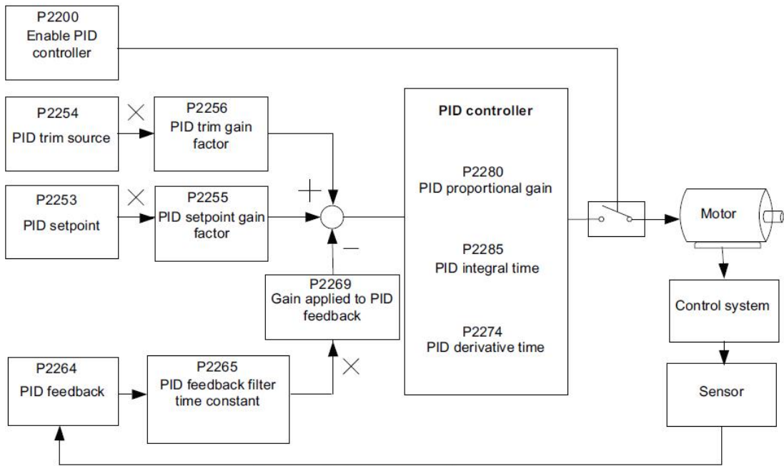
Related parameters for PID controller
