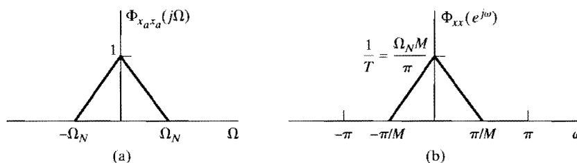
Figure 4.67 Illustration of frequency and amplitude scaling between \Phi_{x_a x_a}(j\Omega) and \Phi_{xx}(e^{j\omega}) .
