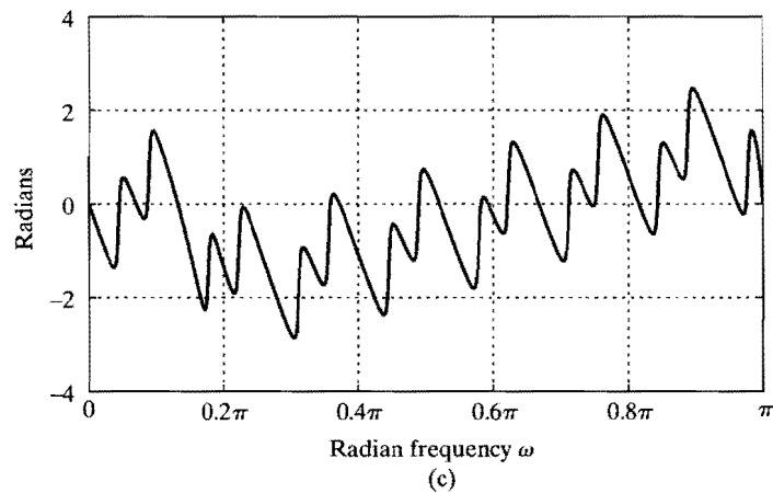
Figure 13.13 Fourier transforms of x[n] in Figure 13.10. (a) Log magnitude. (b) Principal value of the phase. (c) Continuous “unwrapped” phase after removing a linear-phase component from part (b). The DFT samples are connected by straight lines.
