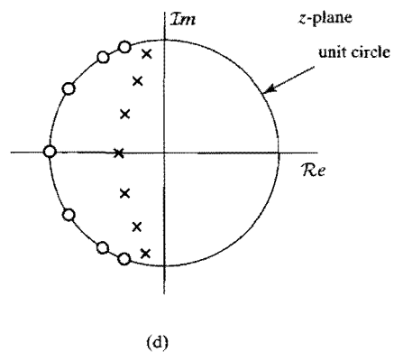
Figure 7.14 Chebyshev Type II filter, 7 th -order.
