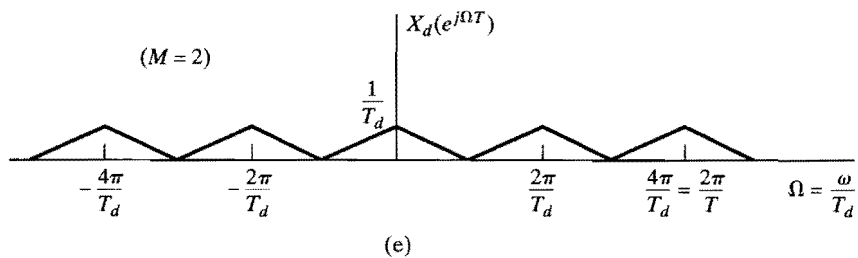
Figure 4.20 Frequency-domain illustration of downsampling.
