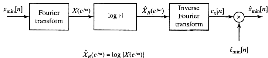
Figure 13.2 Determination of the complex cepstrum for minimum-phase signals.
