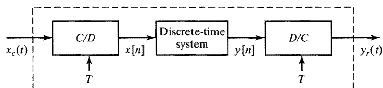
Figure 4.10 Discrete-time processing of continuous-time signals.
