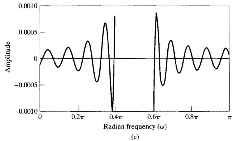
Figure 7.34 Response functions for the lowpass filter designed with a Kaiser window. (a) Impulse response ( M = 37 ). (b) Log magnitude. (c) Approximation error for A_e(e^{j\omega}) .
