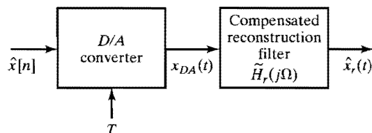
Figure 4.64 Physical configuration for D/A conversion.
