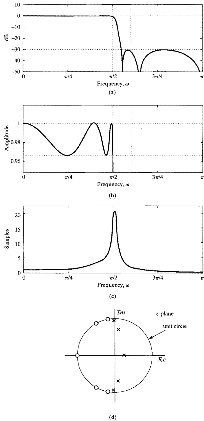
Figure 7.15 Elliptic filter, 5 th -order, exceeds design specifications.
