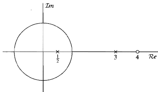
Figure P5.24 Pole-zero diagram for H(z) .
