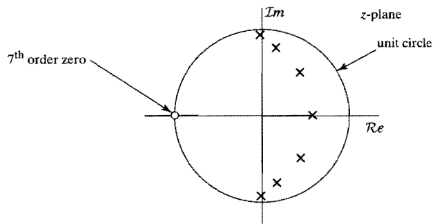
Figure 7.13 Chebyshev Type I filter, 7 th -order.
