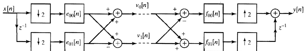
Figure 4.46 Polyphase representation of the two-channel analysis and synthesis filter bank of Figure 4.44.
