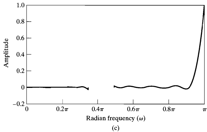
Figure 7.36 Response functions for type II FIR highpass filter. (a) Impulse response ( M = 25 ). (b) Log magnitude of Fourier transform. (c) Approximation error for A_e(e^{j\omega}) .
