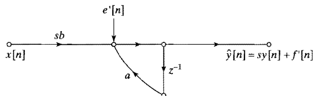
Figure 6.63 Scaled 1 st -order system.
