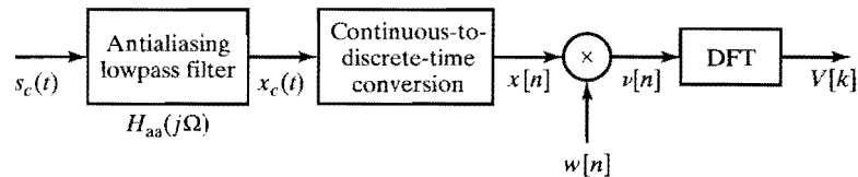
Figure 10.1 Processing steps in the discrete-time Fourier analysis of a continuous-time signal.
