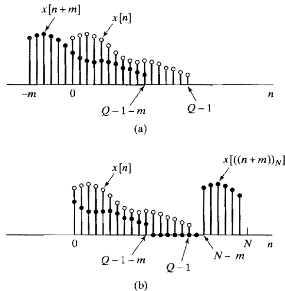
Figure 10.28 Computation of the circular autocorrelation. (a) x[n] and x[n+m] for a finite-length sequence of length Q . (b) x[n] and x[((n+m))_N] as in circular correlation.
