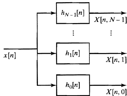
Figure 10.15 Filter bank representation of the time-dependent Fourier transform.
