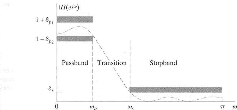
Figure 7.1 Lowpass filter tolerance scheme.
