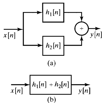
Figure 2.11 (a) Parallel combination of LTI systems. (b) An equivalent system.
