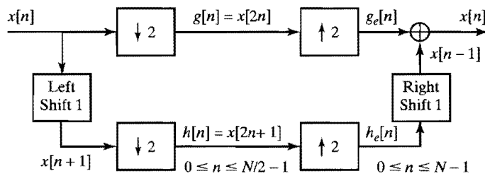
Figure 9.3 Illustration of the basic principle of decimation-in-time.
