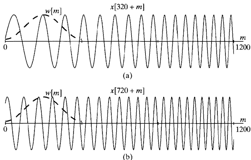
Figure 10.11 Two segments of the linear chirp signal x[n] = \cos(\alpha_0 n^2) for \alpha_0 = 15\pi \times 10^{-6} with a 400-sample Hamming window superimposed. (a) X[\lambda] at n = 320 would be the DTFT of the top trace multiplied by the window. (b) X[\lambda] at n = 720 would be the DTFT of the bottom trace multiplied by the window.
