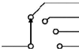
1-pole 4-way switch symbol
